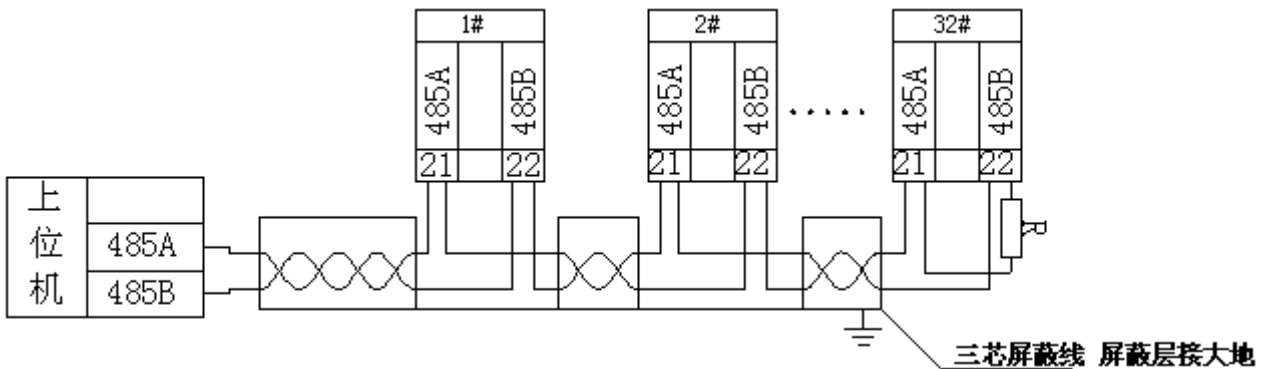
Three-core shielded line/shielding layer is connected with ground.
